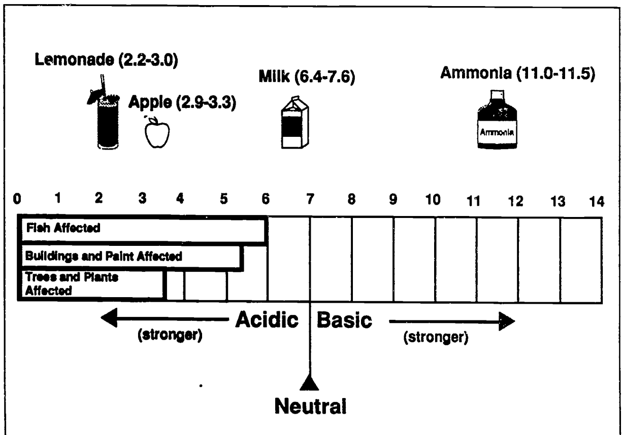
This diagram shows the pH scale. On top are some common items and their pH. A pH stronger than around 5 can harm buildings, metals, paint, and other materials. What pH level can harm fish? How about plants? Are these levels of acidity stronger or weaker than the level that affects materials? See the next page to learn more about pH.
